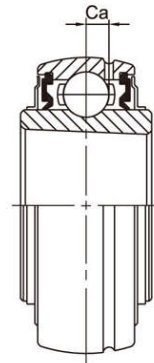
SUK200G Relubricatable type
