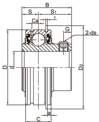
SL TYPE SEAL
