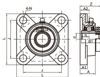
SSUEF200EHB(Hollow Base)
