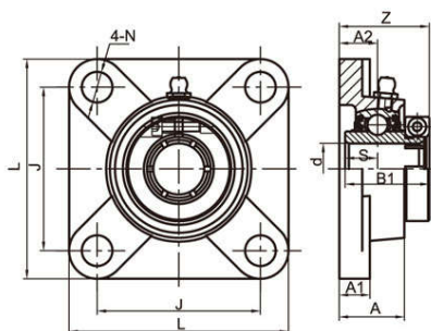
SSUEF200ESB(Solid Base)
