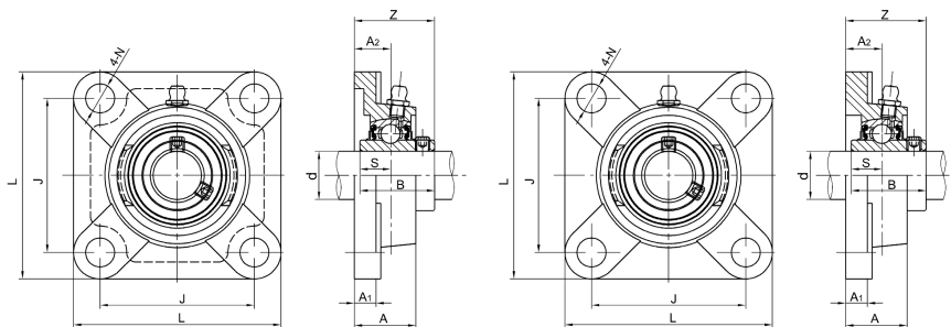
• SSUCF200EHB (空心底)
