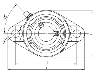
• SSUCFL200EHB (空心底)
